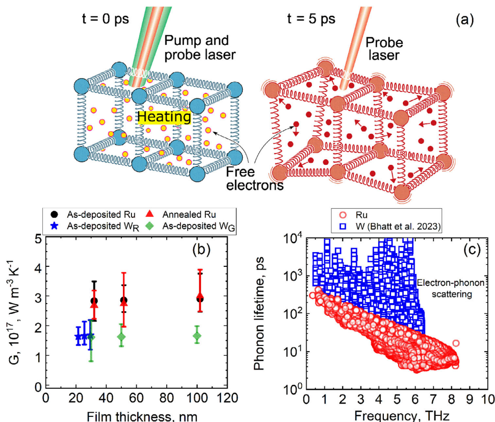
Figure 4. a) The electron–phonon scattering mechanism under the laser excitation. b) Two temperature model derived electron–phonon coupling factor ( G ) of the as-deposited films. The measured coupling factor of Ru is higher than that of W, indicating that more electron–phonon scattering events occur in Ru, which results in shorter phonon lifetime in Ru as found from our first-principles calculations as shown in (c).
