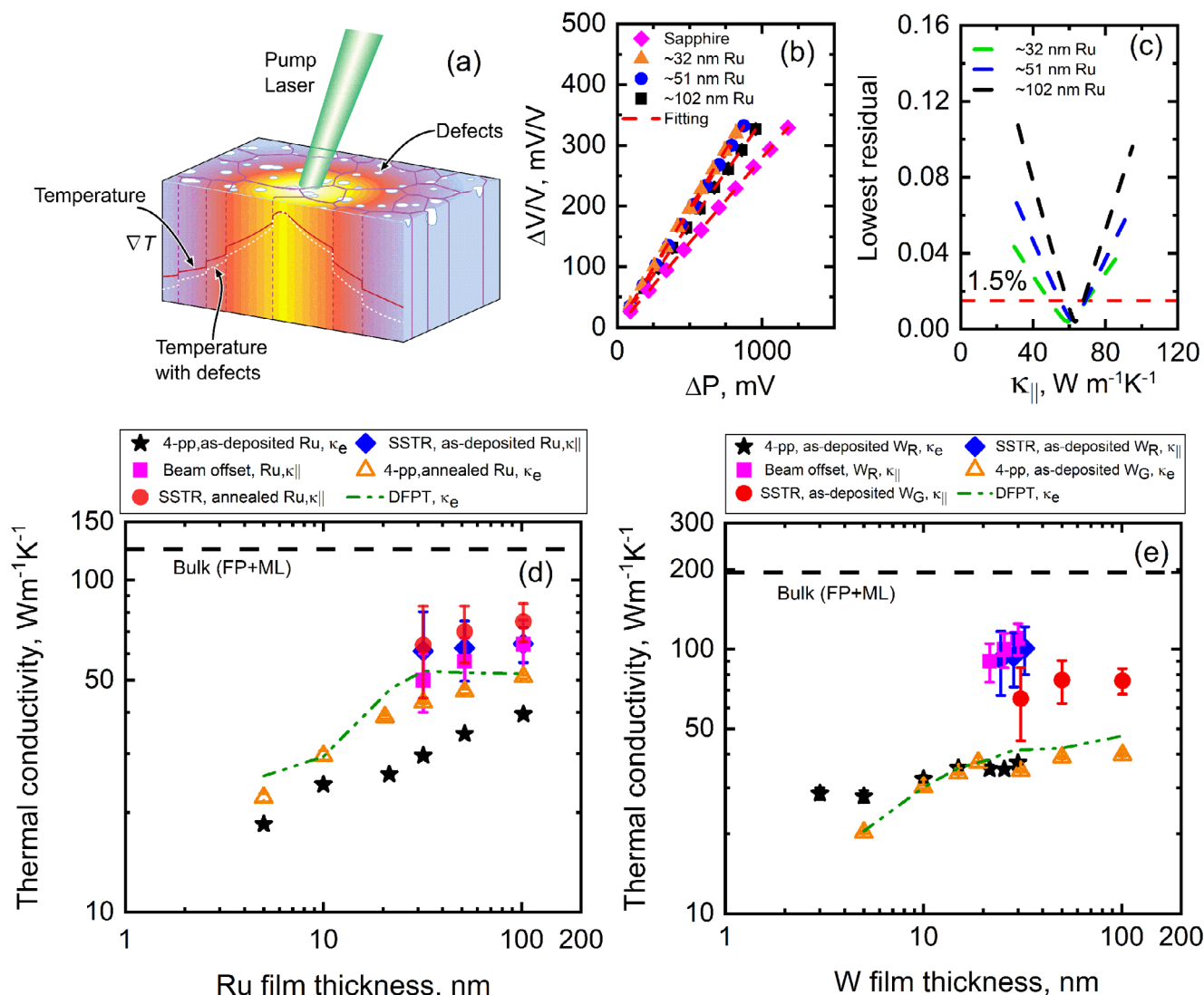
Figure 2. a) Schematic illustrating in-plane heat spreading during an SSTR experiment. Grain boundaries and defects scatter electrons and phonons, impeding heat flow and leading to a higher temperature rise near the pump laser spot and a steeper temperature gradient ( \nabla T ) compared to an ideal defect-free material. The dashed line represents the modified temperature profile caused by defects. b) Plot of \frac{\Delta V}{V} vs. \Delta P (where \Delta P \propto pump power) used in the SSTR fitting to extract the thermal conductivities of Ru films. c) 2D contour analysis of Ru films with different thicknesses, assuming the quality of fit between model parameters and experimental data is within a 1.5% threshold value. d,e) In-plane thermal conductivity ( \kappa_{||} ) of the as-deposited Ru and W films measured with SSTR, shown by blue diamond symbols. The SSTR-measured in-plane thermal conductivity of the as-deposited Ru and W films is higher than that derived from the Wiedemann–Franz law applied to electrical resistivity measurements (indicated by the star symbol), assuming the low-temperature Lorenz number. This difference arises from the phonon contribution to the thermal conductivity of Ru ( 27.4 \pm 3.0 \text{ W m}^{-1} \text{ K}^{-1} , determined using a machine-learned potential developed from ab initio molecular dynamics simulations) and W ( \approx 60 \text{ W m}^{-1} \text{ K}^{-1} ). [9] The short-dashed line indicates the predicted electron thermal conductivity of Ru and W thin films as a function of film thickness. The intrinsic bulk electron thermal conductivity, obtained from density functional perturbation theory (DFPT), is modified to account for boundary scattering (arising from finite film thickness and grain size), point defect scattering, and electron–phonon interactions through Matthiessen’s rule. While the model exhibits strong agreement with experimental data for W, it slightly overestimates the values for Ru, which is attributed to mixed grain morphology not fully captured by the current modeling framework.
