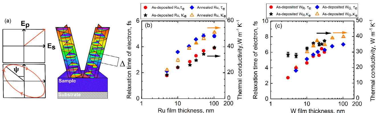
Figure 3. a) Schematic representation of spectroscopic ellipsometry for thin film characterization. b) The effective relaxation time of as-deposited Ru (represented by red circle symbols) determined from IR-VASE measurements exhibits a thickness-dependent trend that aligns with the behavior of electron thermal conductivity. For annealed Ru films, the relaxation time increases due to the larger length scale of electron-grain boundary interaction. c) Similarly, the effective relaxation time for as-deposited W_R and pure W_G films follows a size-dependent trend, consistent with data obtained from 4-point-probe measurements.
