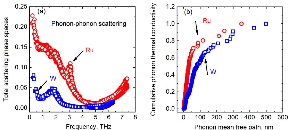
Figure 5. a) Total phonon–phonon scattering phase space (SPS) as a function of phonon frequency for Ru (red circles) and W (blue squares). The significantly larger SPS in Ru indicates higher phonon–phonon scattering rates, contributing to reduced phonon lifetimes and lower thermal conductivity compared to W. b) Normalized cumulative phonon thermal conductivity as a function of phonon mean free path for Ru (red circles) and W (blue squares). In Ru, a substantial fraction of the phonon thermal conductivity arises from phonons with mean free paths below ~50 nm, whereas in W, phonons with longer mean free paths contribute more significantly.
