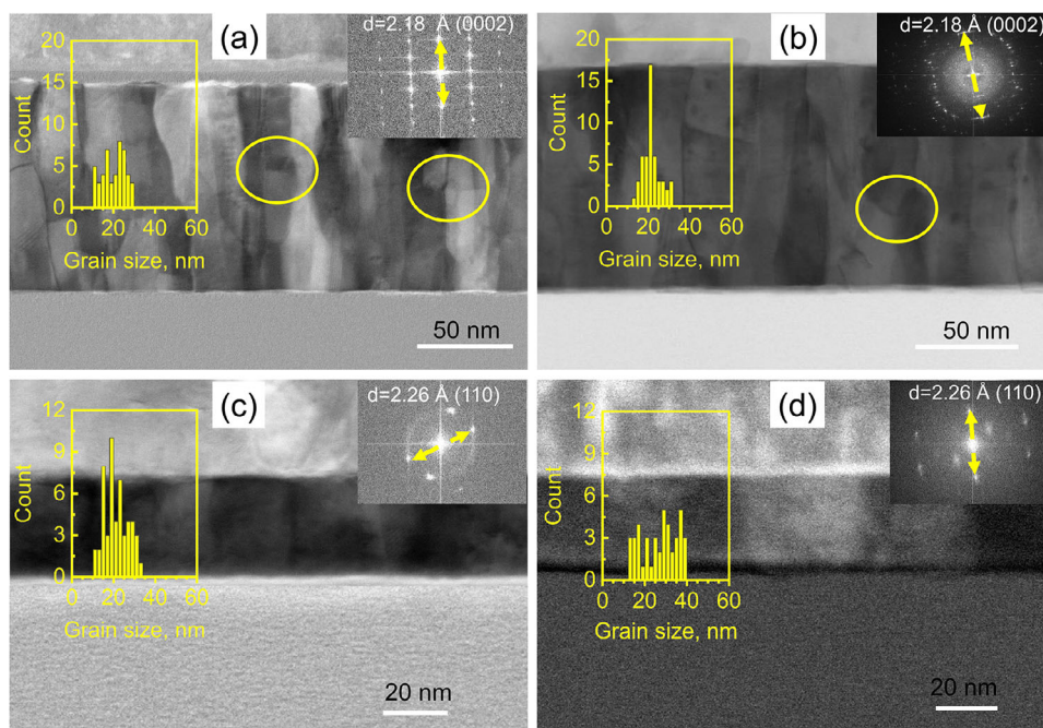
Figure 1. STEM image of a) as-deposited \approx 102 nm Ru, b) 400^\circ\text{C} annealed \approx 102 nm Ru films, c) as-deposited \approx 30 nm \text{W}_\text{R} , and d) as-deposited \approx 31 nm \text{W}_\text{C} , respectively. The micrographs show the representative area of the as-deposited films. The insets show the grain size distributions as raw histograms, without assuming any particular statistical model. Ru exhibits a mixed grain morphology where the dominant structure is columnar, but some grains exhibit irregular or equiaxed forms (marked by circle). Annealing does not eliminate the mixed grain morphology in the Ru films, but it increases the proportion of larger grains. The grains of W films are mostly columnar. The FFT patterns obtained from selected regions of the high-resolution STEM of these as-deposited films confirm the HCP structure of Ru and the BCC structure of W.
